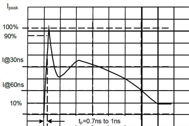
Figure 4. IEC 61000-4-2 Waveform
