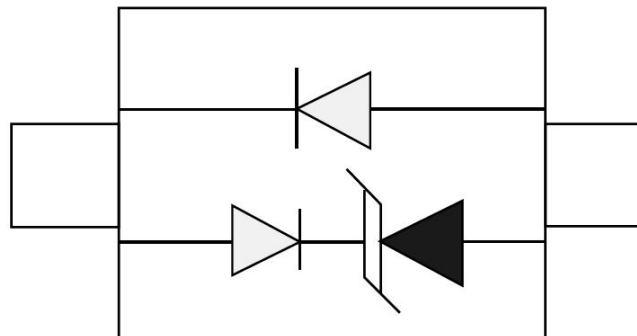
DFN-2L (Top View)
