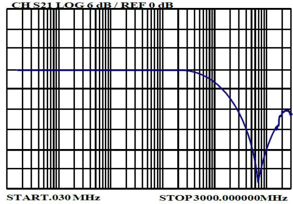
Figure 2: Insertion Loss
