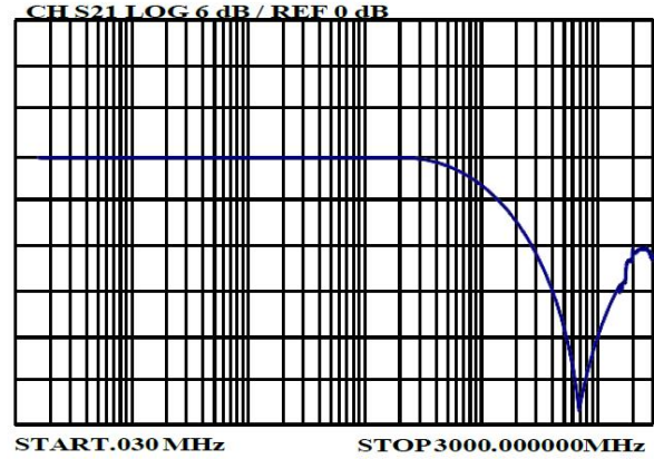
Figure 2: Insertion Loss
