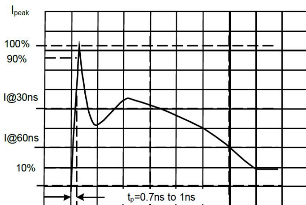
Figure 4. IEC 61000-4-2 Waveform
